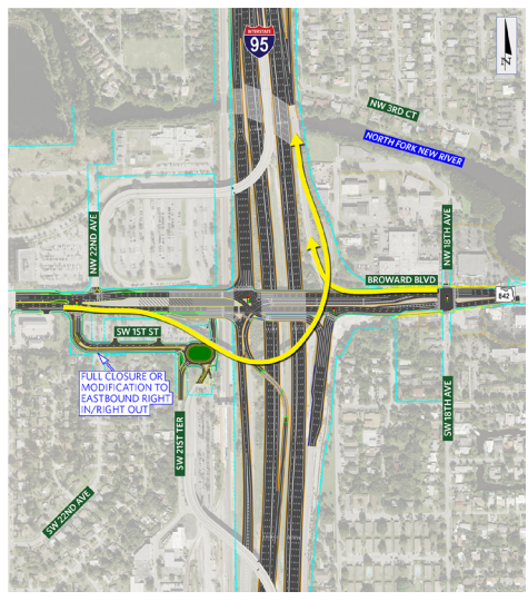
I-95 NB GENERAL PURPOSE ENTRANCE
