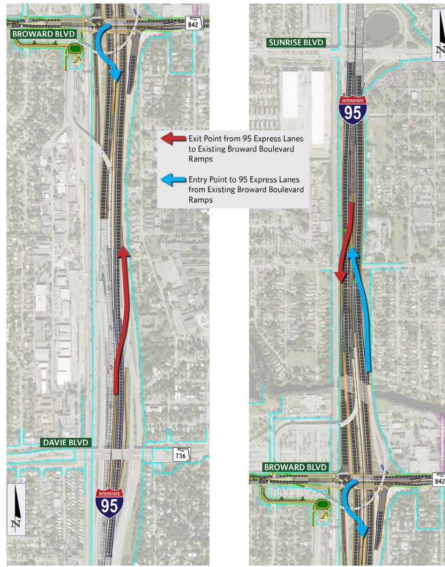
95 EXPRESS CONNECTIVITY WITH BROWARD BLVD
